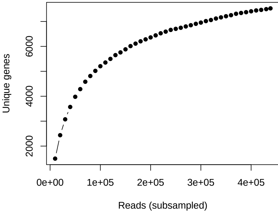
Gene saturation
