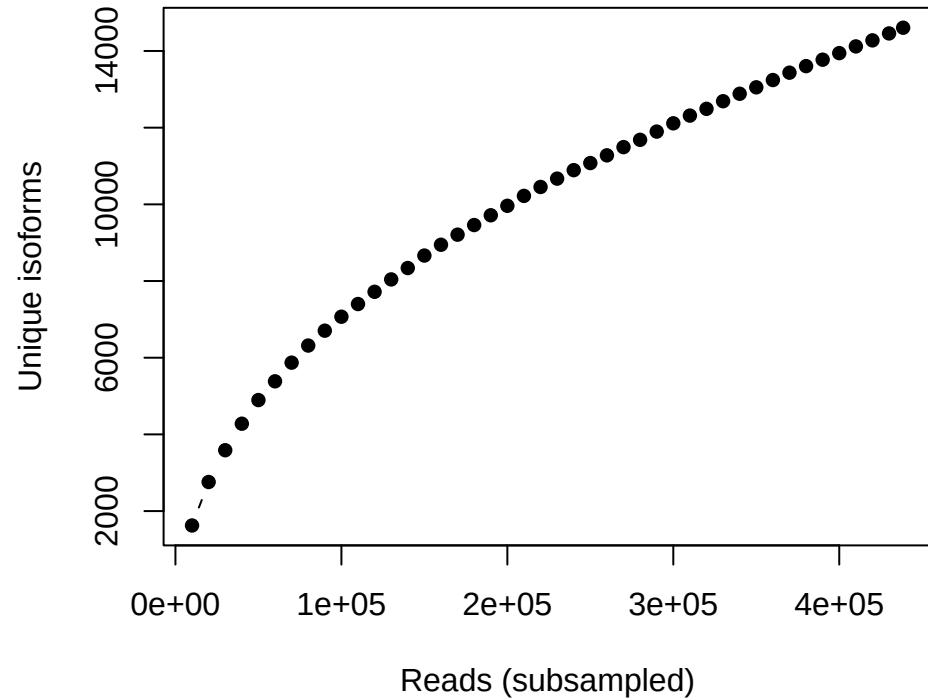
Isoform saturation
